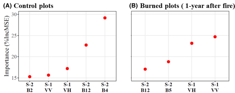
Figure 4. Relative variable importance in Random Forest models measured as the percentage increase in mean square error (%IncMSE), in unburned control plots (A) and burned plots 1 year after fire (B).
